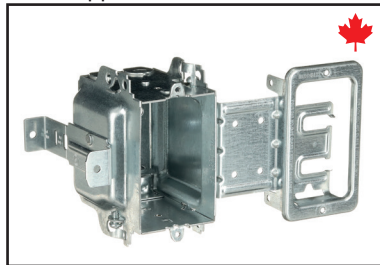
Iberville® Gangable boxes with low-voltage cable support bracket
